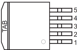
MIC29502WU(TO263-5)
