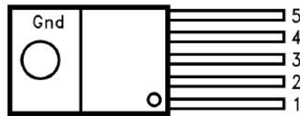
MIC29502WT(TO220-5)
